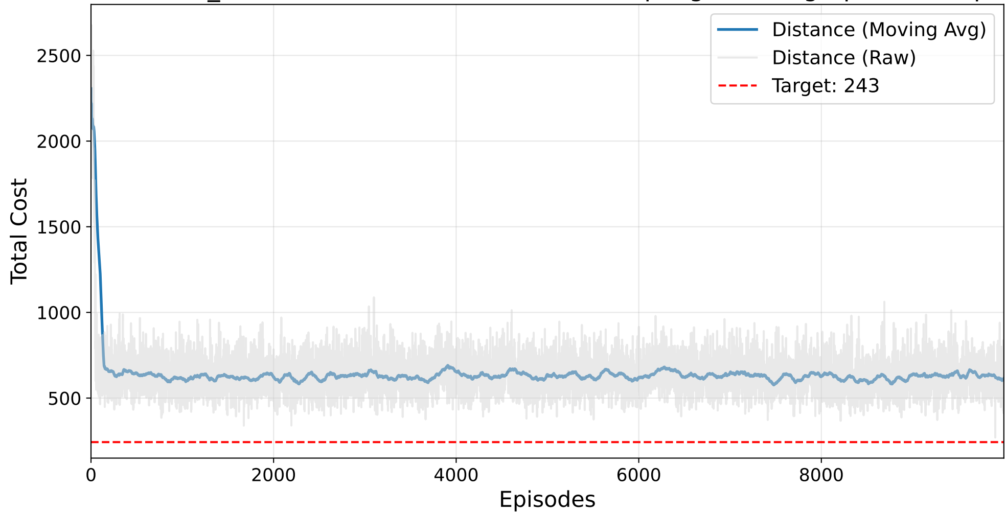
Final NO_MASK Masked AutoRL-SOP (Resampling) Training - prob.42.sop
